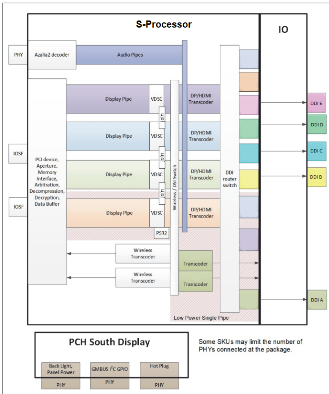
Figure 17. S Processor Display Architecture
