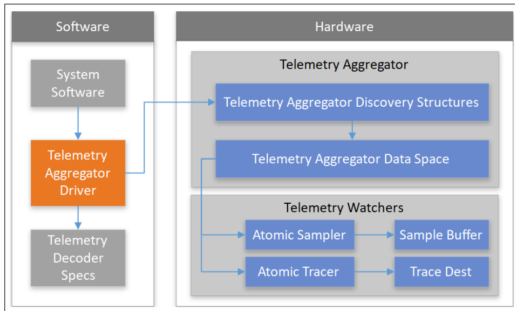
Figure 6. Telemetry Aggregator
