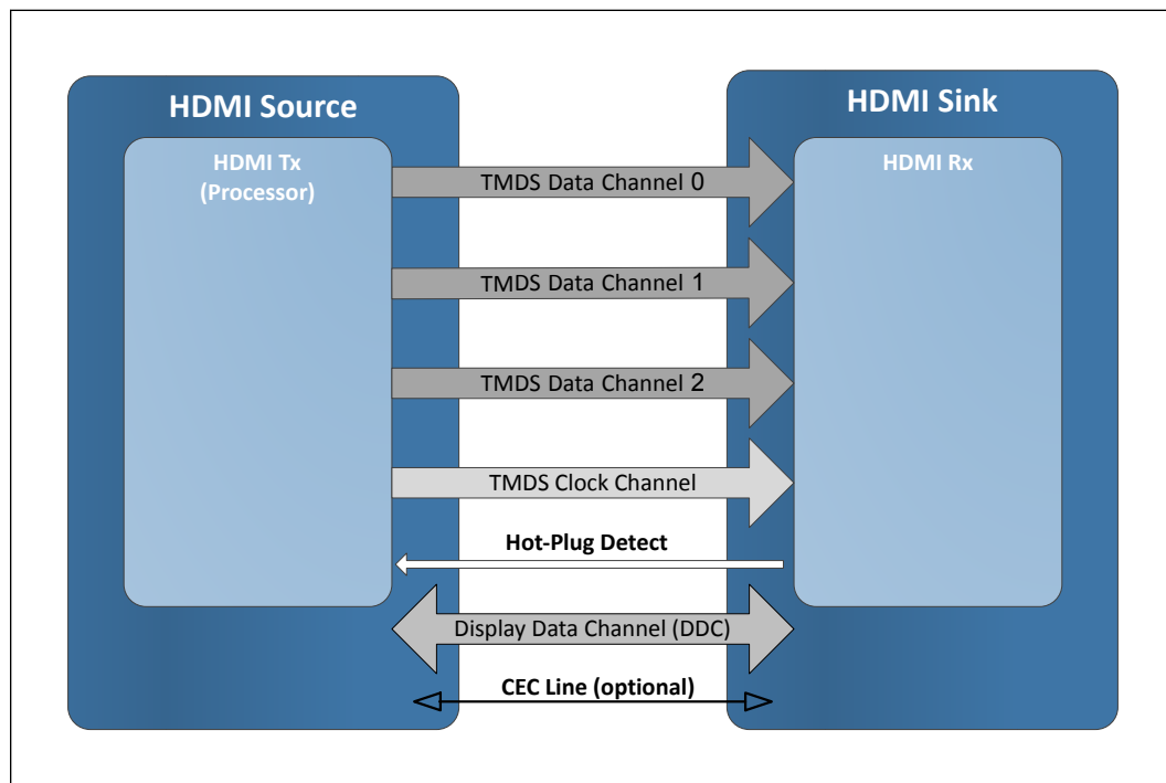
Figure 19. HDMI* Overview
