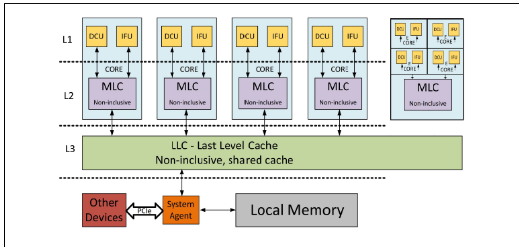
Figure 5. Hybrid Cache
