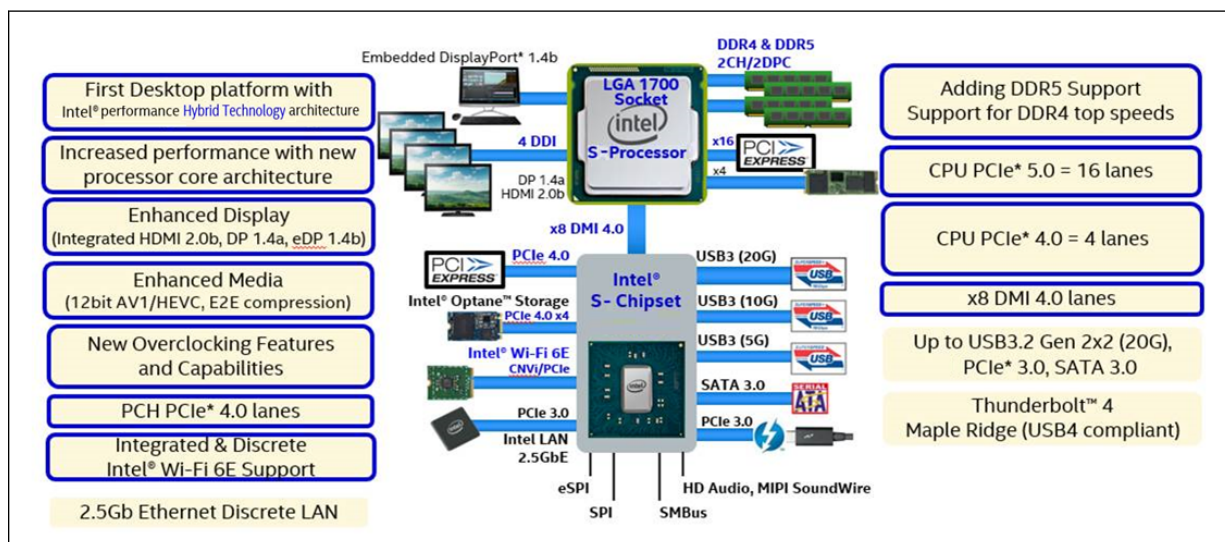
Figure 1. S Processor Line Platform Diagram
