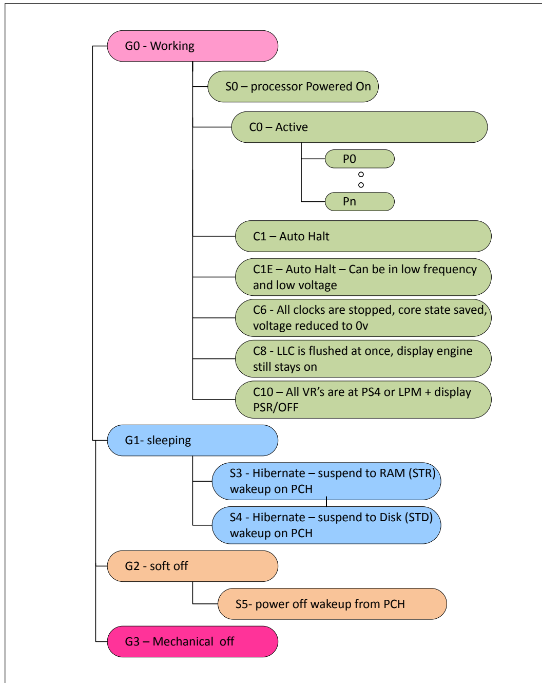
Figure 7. Processor Power States
