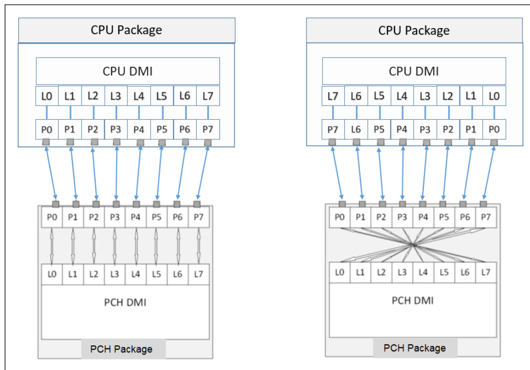
Figure 16. Example for DMI Lane Reversal Connection
